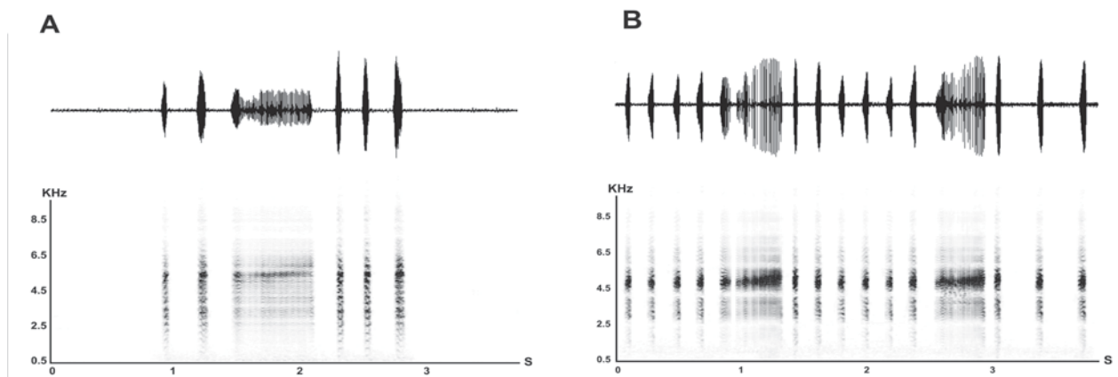
Fig. 2. Oscillogram and spectrogram of a call fragment of (A) Scinax aromothyella , and (B) S. berthae
